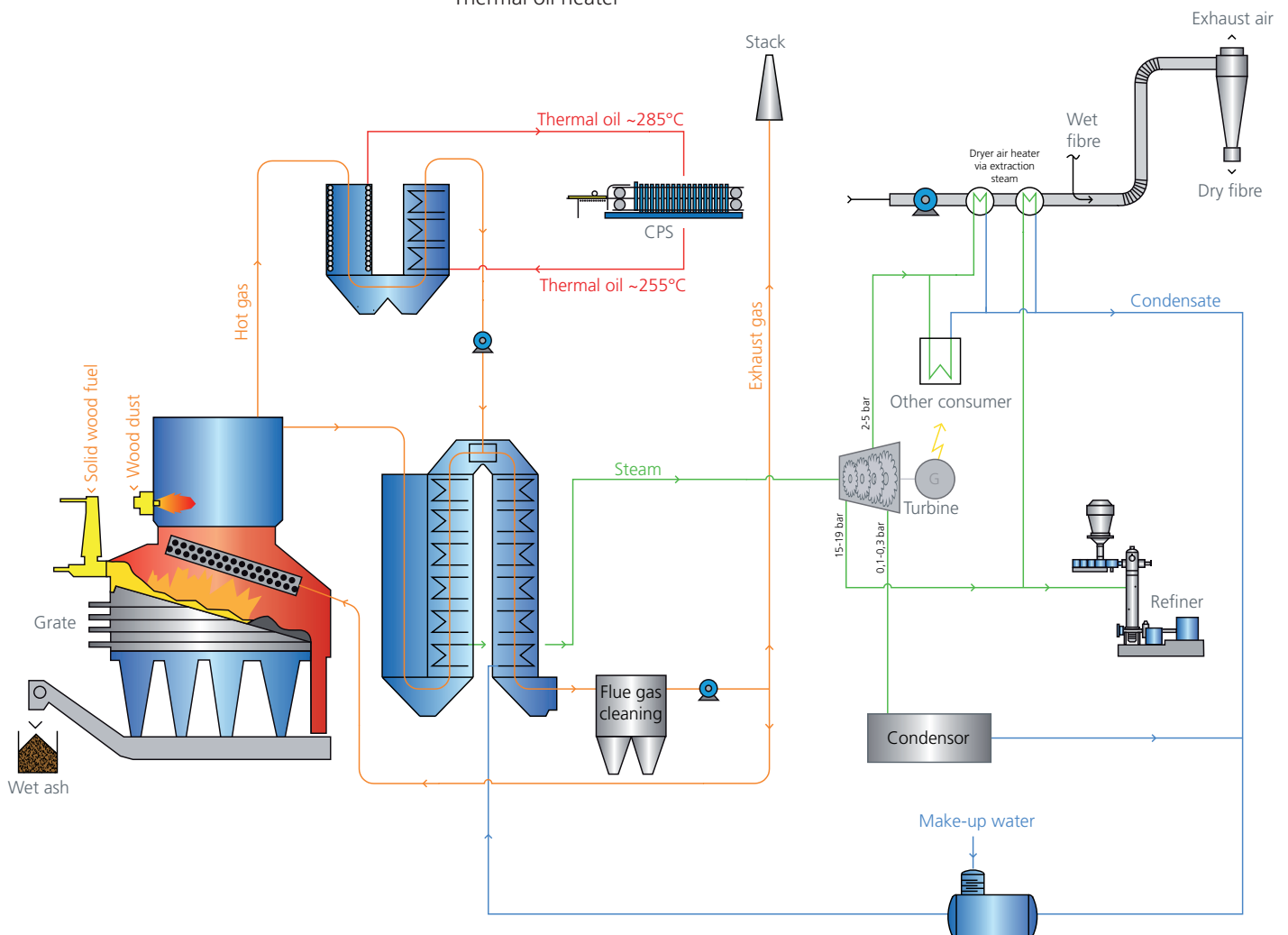
Example: Co-generation plant integrated in an MDF-plant
