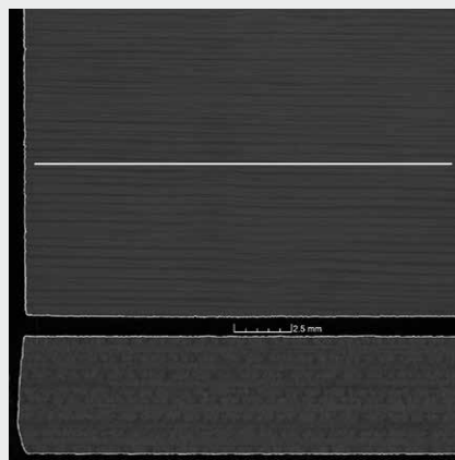
Fibercon consolidation quality Porosity << 1% Perfect fiber alignment
