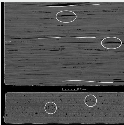
State of the art consolidation quality Porosity < 2% Fiber ondulations
